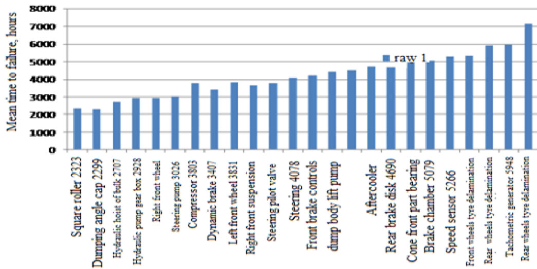
Fig. 1.1. The diagram of the mean time to failure of the main components and assemblies of BelAZ-540A and BelAZ-548A dump trucks
