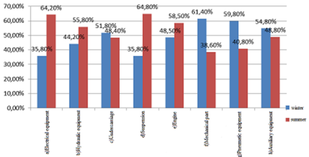
Fig. 1.4. Assessed Failure Rate Distribution Diagram BelAZ-540A and BelAZ-548A dump trucks by periods of operation
