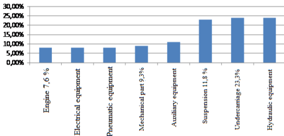
Fig. 1.3. The assessed failure rate Distribution Diagram between subsystems of dump trucks BelAZ-540A and BelAZ-548A
