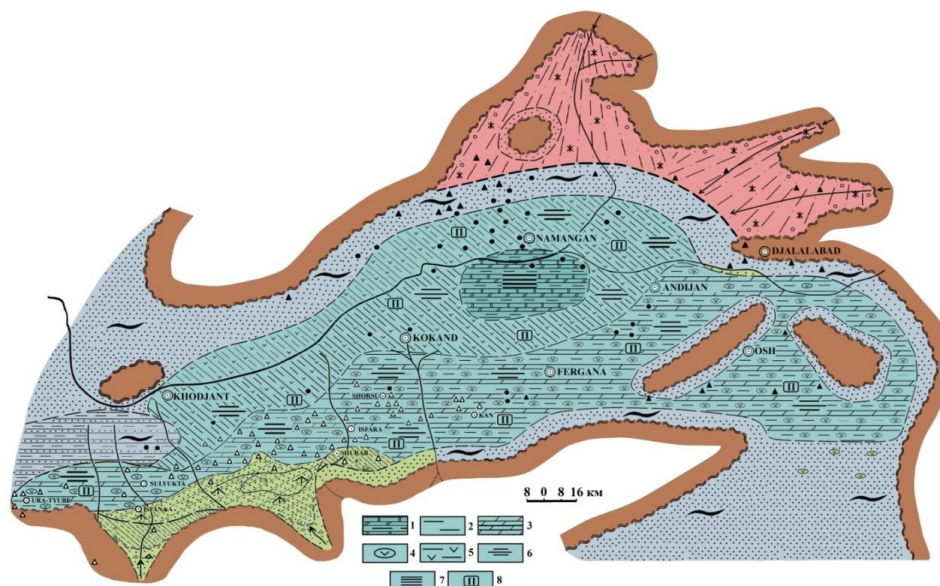
Figure 3. Facial-paleogeographic map of the upper Suzak time of the Paleogene of the Fergana depression.
