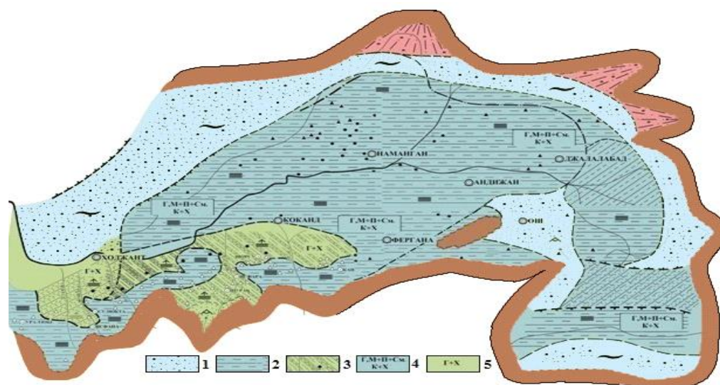
Figure 4. Facies-paleogeographic map of the Samsar time of the Paleogene of the Ferghana Depression (12th rhythm pack).
