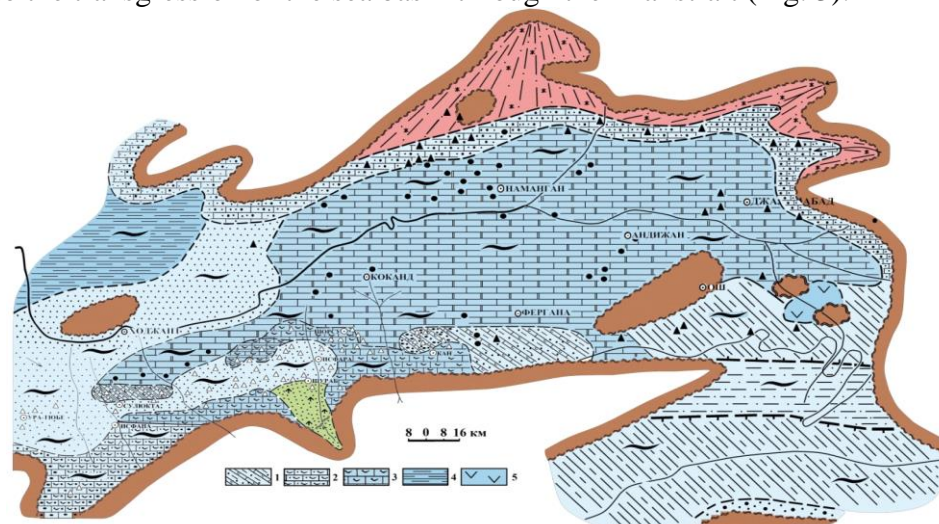
Figure 2. Facies-paleogeographic map of the Middle Suzak time of the Paleogene of the Ferghana basin (4th rhythm pack).
