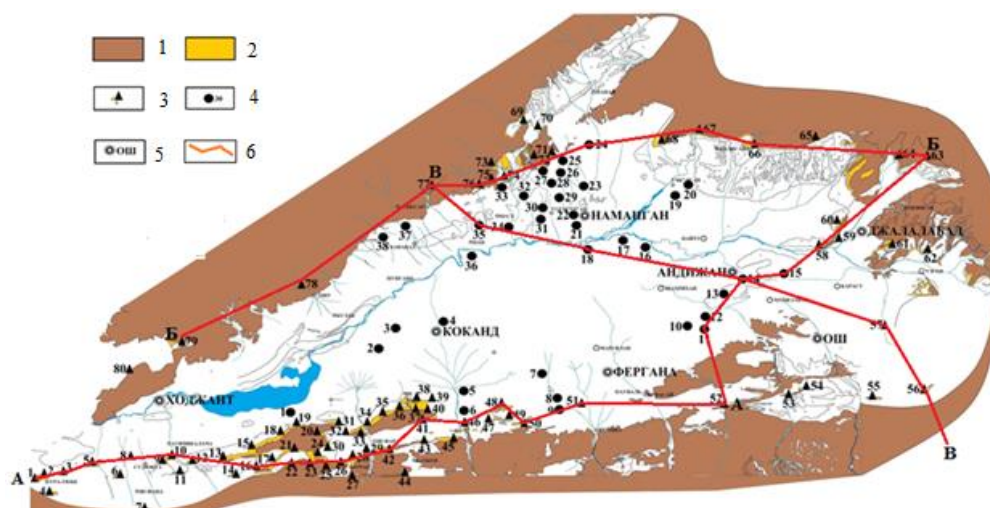
Figure. 1. Map of factual material (compiled by the author on the basis of a geological map of scale 1: 200000).
