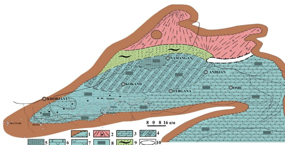
Figure. 3. Facial-paleogeographic map of the Bukhara time of the Paleogene of the Fergana depression (the gypsum formation of Goznau).
