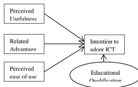
Figure 1: Proposed Model
