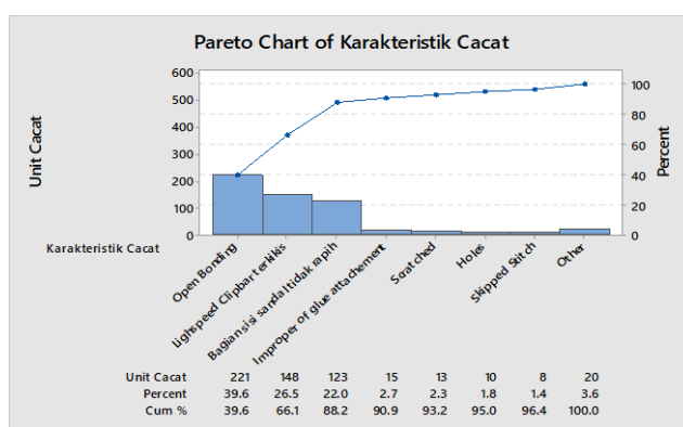
Figure 1 Pareto diagram of 11 types of defects
