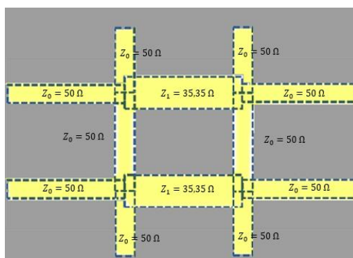
Fig 3. Hshape Junction with Impedansi
