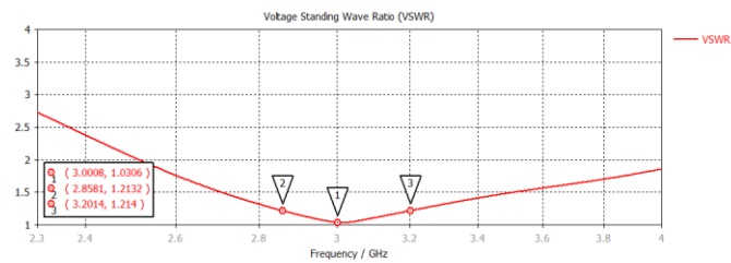
Fig 9. Simulation Result of Vswr H Shape Junction
