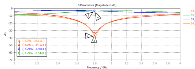
Fig 6. SimulaionResul From Calculation J Junction
