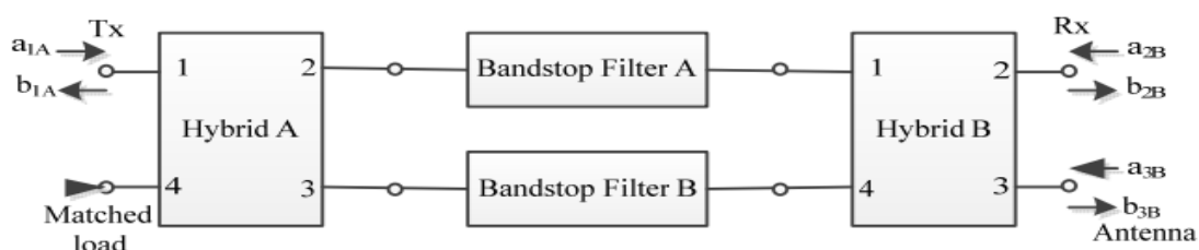
Fig 1. Duplexer
