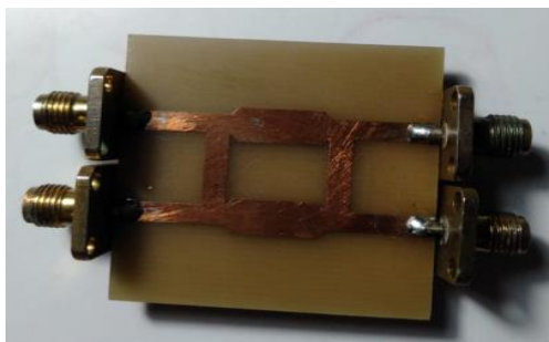
Fig 4. Branchline Coupler JShape Junction
