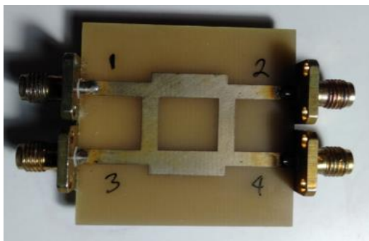
Fig 2. Branchline Coupler H Shape junction
