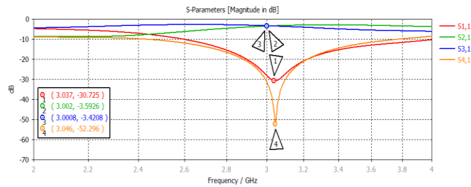
Fig 8. Simulation Result Branch Line Coupler J Shape Junction
