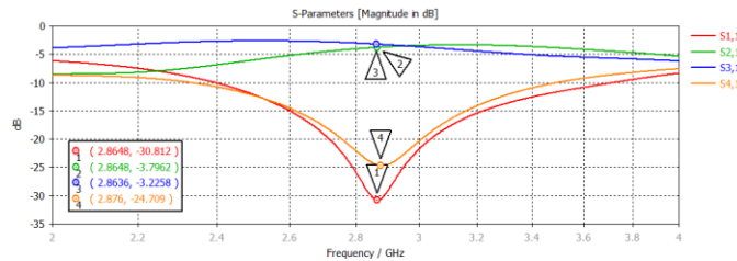
Fig 5. SimulaionResul From Calculation H Junction
